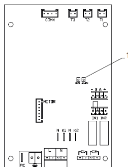
1 = LED kontrolka
